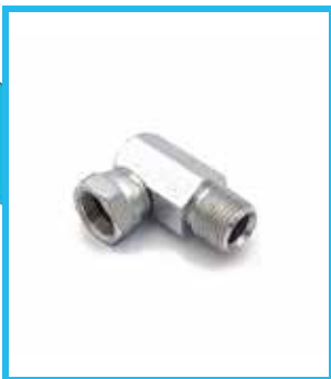
Macnaught Retractable Oil Reel 1/2" 90 Degree Swivel PN# 3270-051
